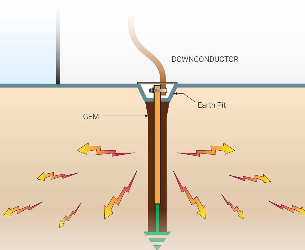
A typical grounding system.
