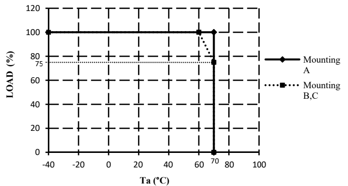
OUTPUT DERATING vs AMBIENT CURVE
