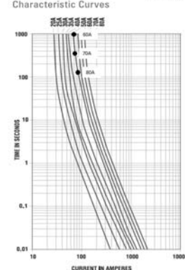
Time-Current Characteristic Curves 0299050_
