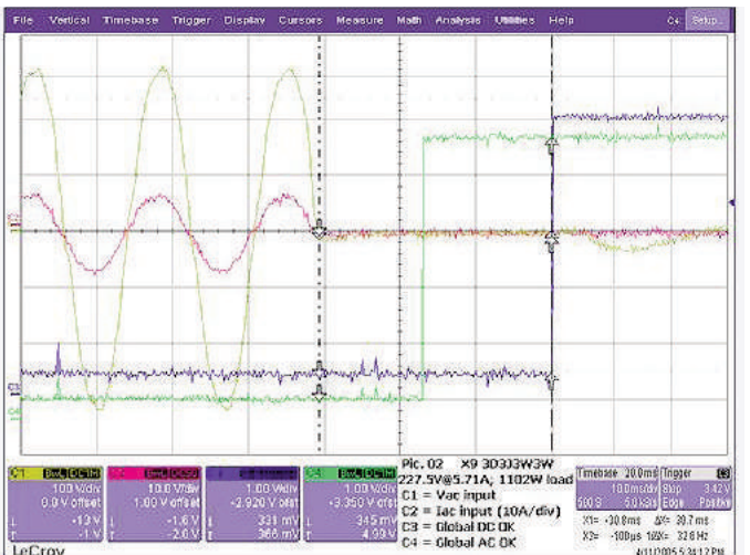
Hold Up Time X9 with 1100 W load
