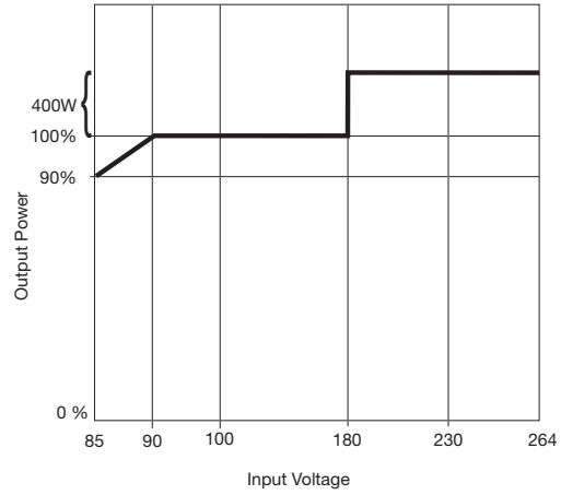
Load derating curve for X4DD, X5DD, X7DD, X9DD and X10DD
