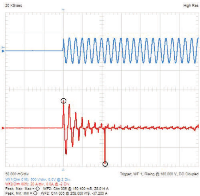
Plot 8. Inrush current for X15 at 230 VAC
