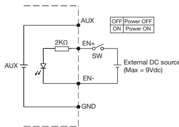
(C) Using external voltage source
