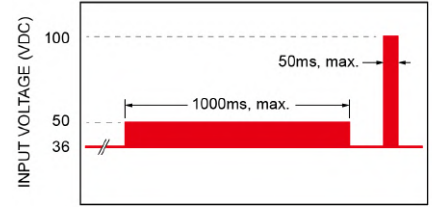
Transient Limitation
