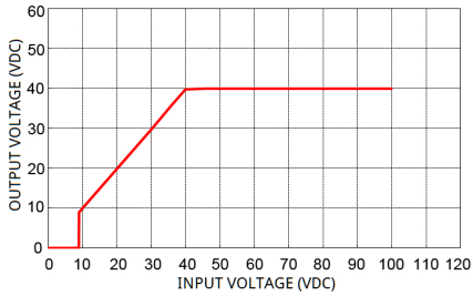
Transfer Function
