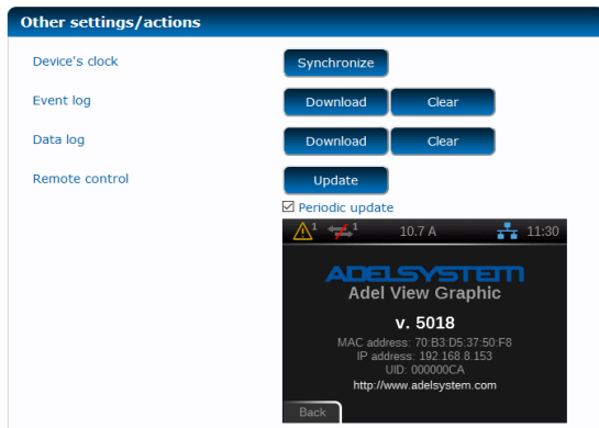
Fig. 9 – Other settings/actions of parameters with the remote control active
