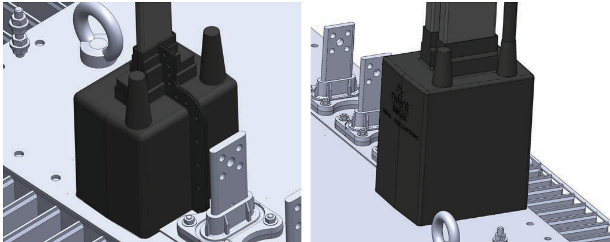
Boot 508160. For one FleXbus Conductor per phase. Typically for power supply applications from 400 kVA to 1600 kVA.
