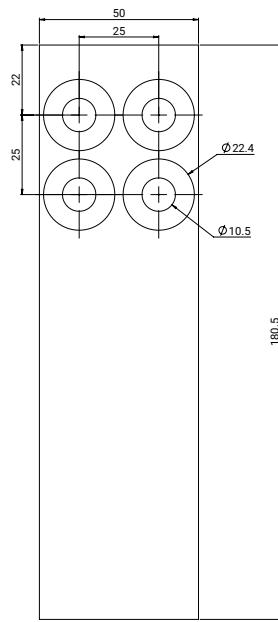
508114: Flexbus Extension 50x10 for conductor 640 mm 2 Type 2
