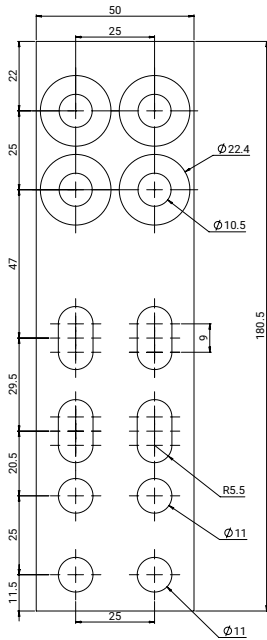
508113: Flexbus Extension 50x10 for conductor 640 mm 2 Type 1
