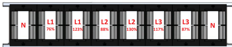
Non-Optimized Conductor Arrangement (Load current unbalanced)
