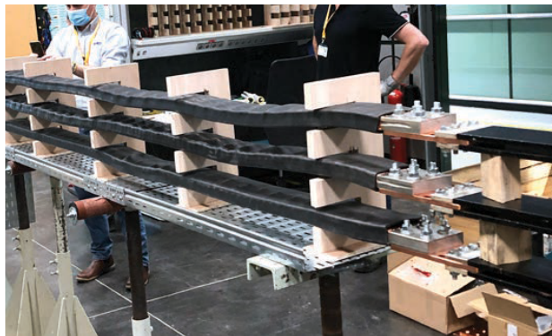
Temperature rise test sequence pictures and probe/temperature sensor all along the installation
