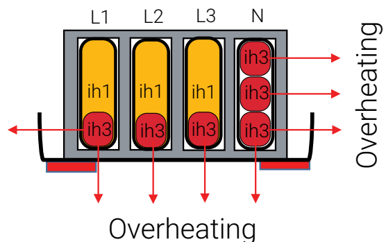
ih3: +33% third order harmonics (150 Hz)
