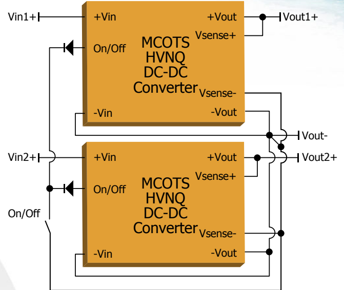
Figure B: Negative output setup
