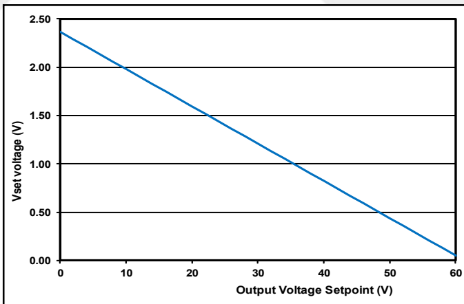
Figure 9: Vset pin voltage vs. Output Voltage Setpoint.
