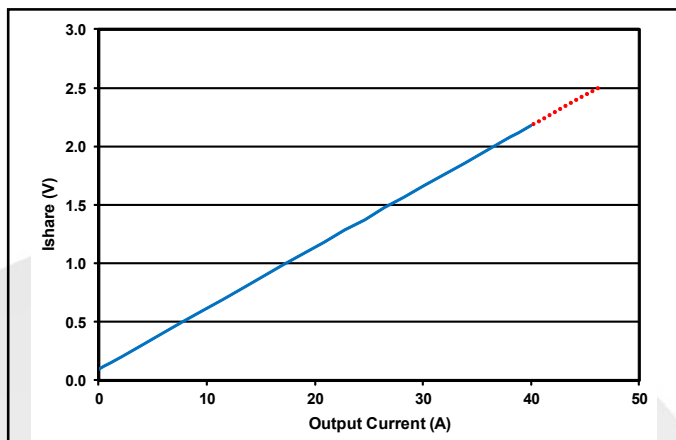
Figure 13: Ishare/Vmon pin Voltage vs. Output Load Current.
